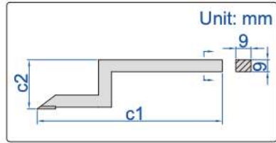
scraper (included)
