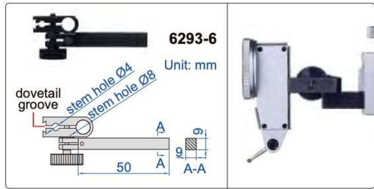
dial test indicator holder (optional)
